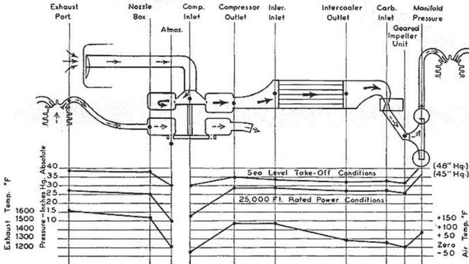
SUPERCHARGER PRESSURE AND TEMPERATURE CYCLE
