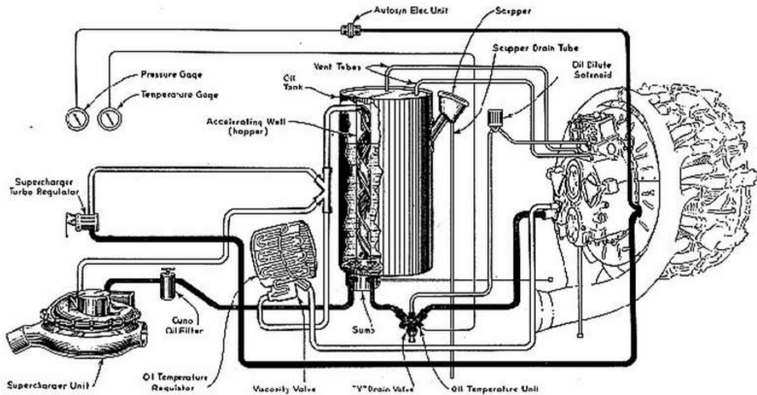
OIL SYSTEM B-24D
