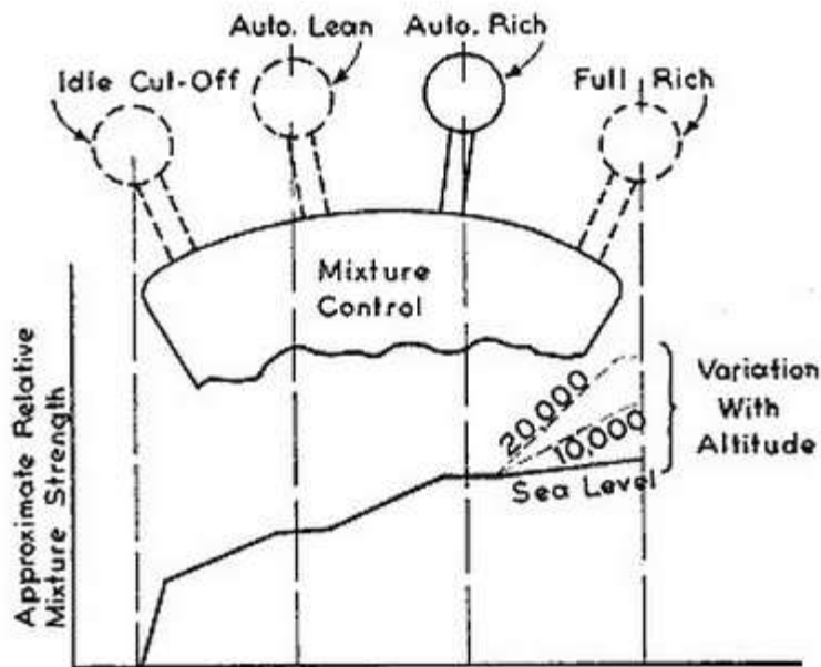
DIAGRAM OF MIXTURE CONTROL QUADRANT Figure One
