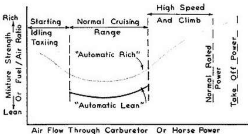
TYPICAL CARBURETOR PERFORMANCE CURVE Figure Two
