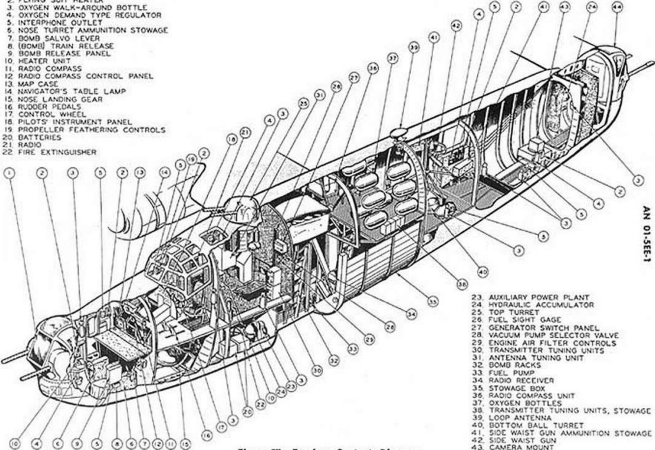
Figure 57—Fuselage Contents Diagram
