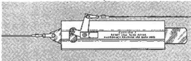
Emergency Bomb Door Cam - Set Position
